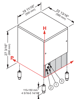
Pieds ajustables 4 5/16" – 5 14/16"
