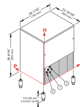
Pieds ajustables 4 5/16" – 5 14/16"
