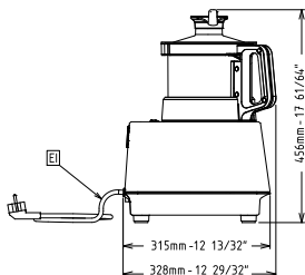
Lateral
