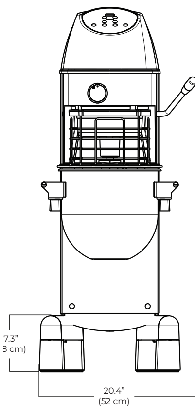
FRONTAL VIEW
