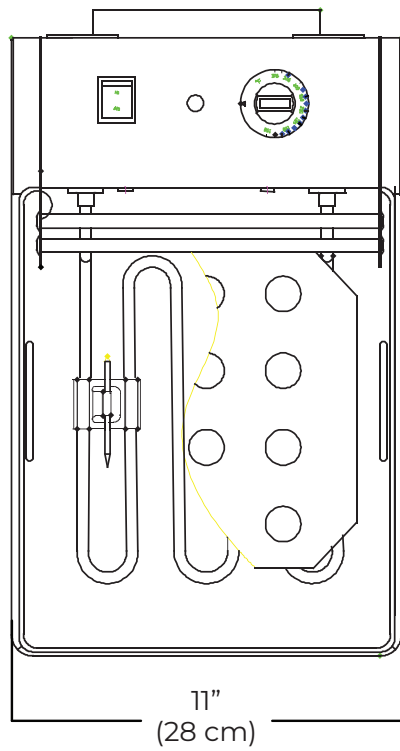
TOP VIEW
