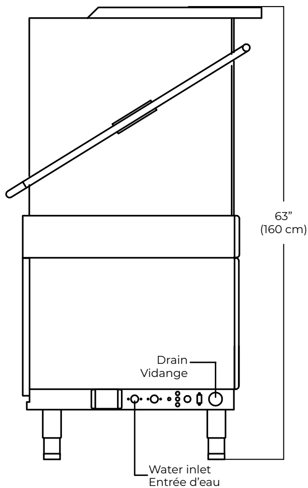
SIDE VIEW
